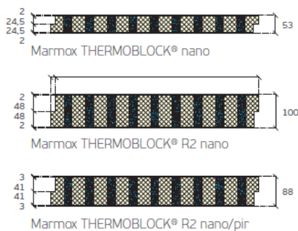
Fig. 2: Different types of Marmox THERMOBLOCK®
