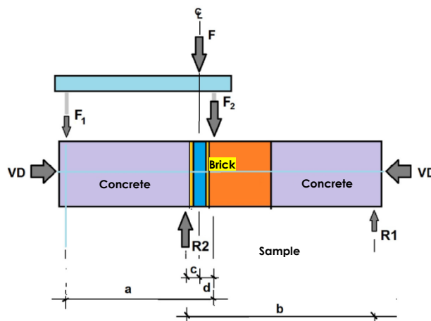
Fig. 4: Configuration for the shear test
